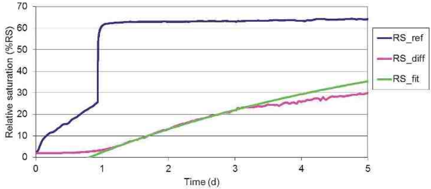
Figure 4. Relative saturation in the measurement line ( RS_{ref} ) and in the side tube ( RS_{diff} ), and best fit of Equation 1 to RS_{diff} (named RS_{fit} ). Distance from sensor head to oil flow is 6.3 cm.
