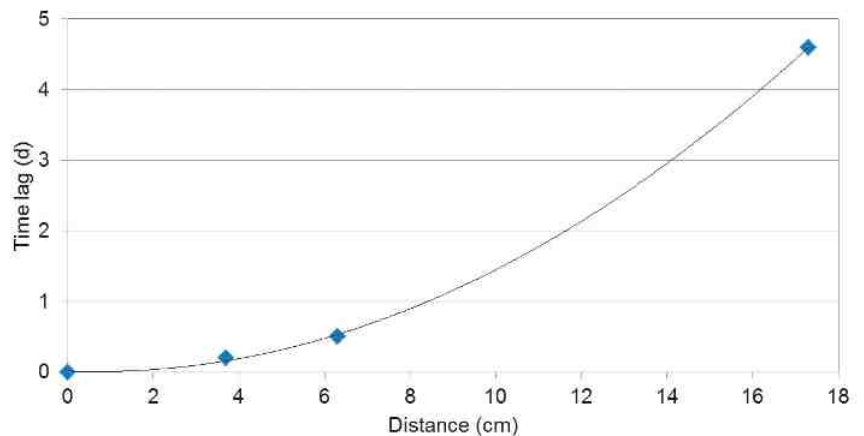
Figure 7. Diffusion time lag t_0 versus moisture sensor distance from oil flow.
