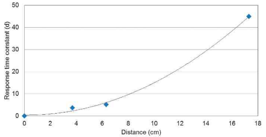
Figure 6. Response time constant \tau versus moisture sensor distance from oil flow.
