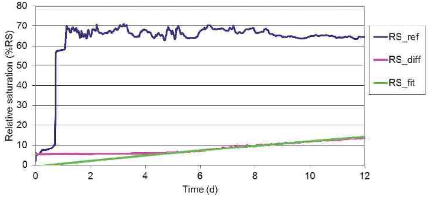
Figure 3. Relative saturation in the measurement line ( RS_{ref} ) and in the side tube ( RS_{diff} ), and best fit of Equation 1 to RS_{diff} (named RS_{fit} ). Distance from sensor head to oil flow is 17.3 cm.
