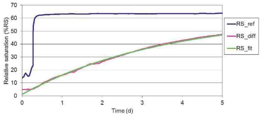
Figure 5. Relative saturation in the measurement line ( RS_{ref} ) and in the side tube ( RS_{diff} ), and best fit of Equation 1 to RS_{diff} (named RS_{fit} ). Distance from sensor head to oil flow is 3.7 cm.
