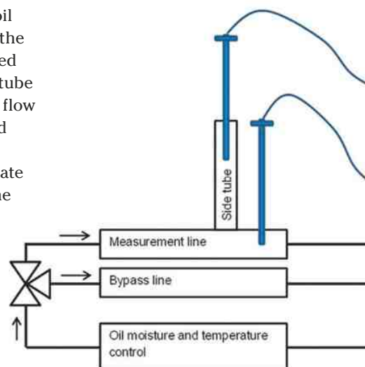
Figure 2. Test setup schematic.
